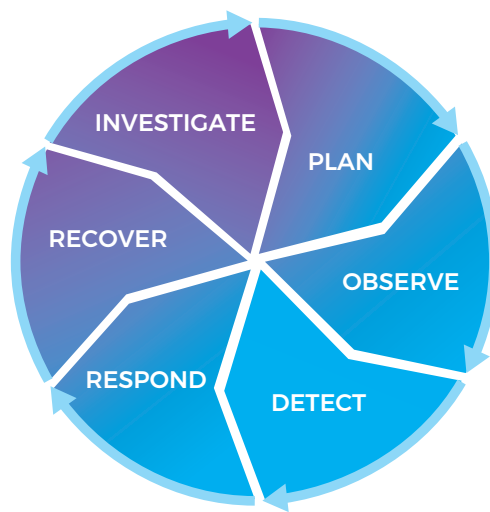
Figure 2: Security Workflow
